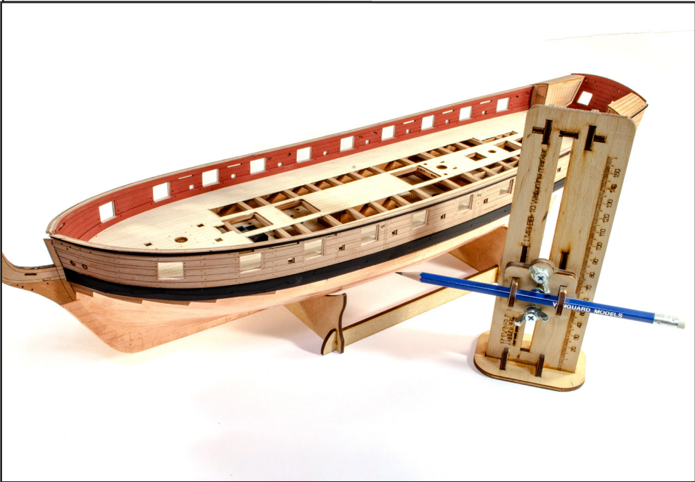
194. Sit the hull in the cradle, making sure the pin in the rear former sits into the hole in the underside of the keel. This makes sure your model is at the right attitude for a waterline to be marked. Use a waterline tool and lightly mark the waterline with the pencil. Check the position of this from the plan and ensure that the tool is at the correct height at bow and stern before you mark.
