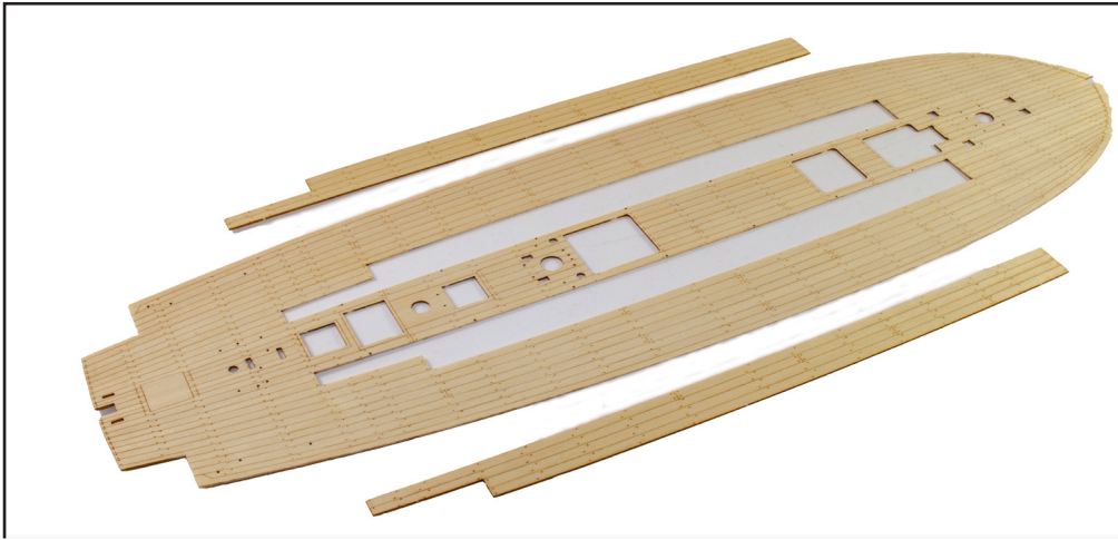
151. You will now need the engraved deck. Remove all the parts which are shown in grey. You can retain the two long portions if you wish to leave the deck complete, or simply not remove them at all.
