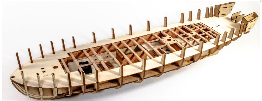
102. This deck now needs to be popped into place. This is very easy and can be done by flexing the deck and hooking it over the bulkhead ears along one side of the hull. As you work the deck downwards so that it locks into the slots at the bottom of those ears, begin to work the opposite side in the same way. The deck should sit in all of those little slots, so if it's not sitting flat the deck, then so around the edges and find the area where the deck isn't slotted in. If correctly slotted, the deck WILL sit perfectly.
