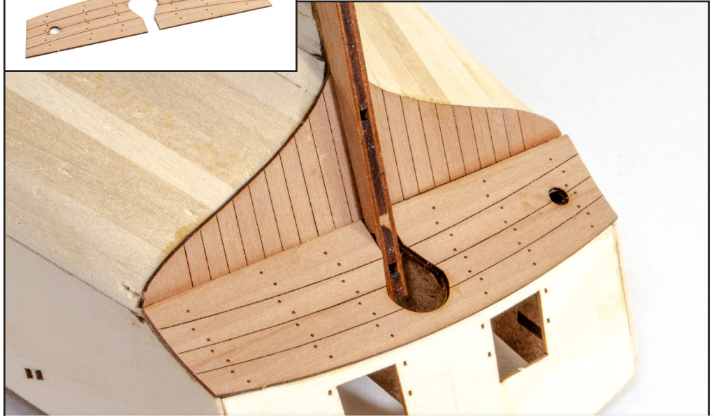
133. Glue part 110 into place as shown. This should naturally sit centrally due to the rudder post parts you just fitted, and the water closet hole on the left should align with the one in the ply level below. There isn't too much of a curve here, so you can just glue and hold this until it dries so you won't need to make pin marks in it. Sand the overhang of this part flush on both sides of the hull.
