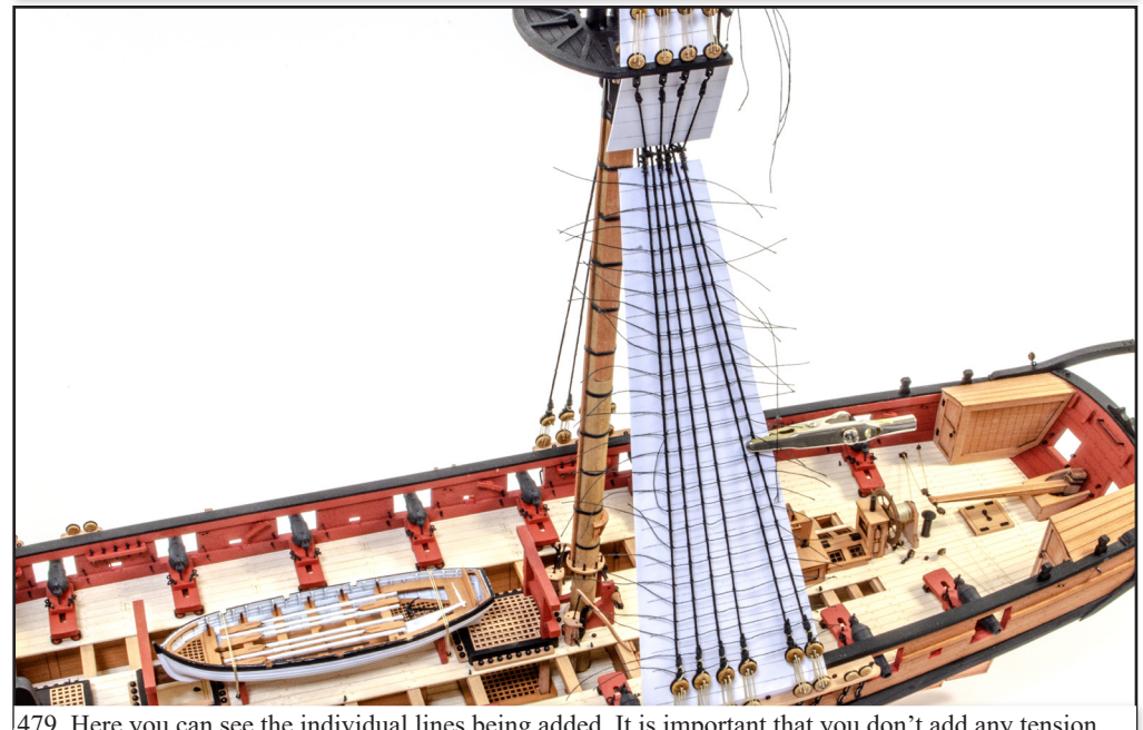
479. Here you can see the individual lines being added. It is important that you don't add any tension into the shroud lines, pulling them out of shape.
