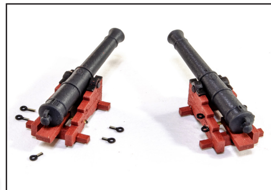
390. Use eyebolts PE-14 to fit into the 5 locations on the cannon carts.
