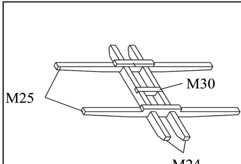
429. Glue together as shown here on the plan sheet. This is the fore mast's trestle tree.
