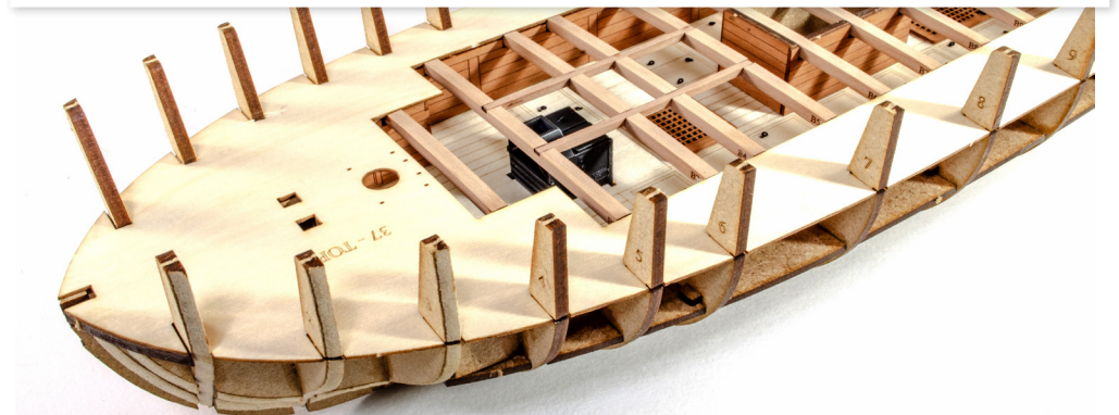
102. This deck now needs to be popped into place. This is very easy and can be done by flexing the deck and hooking it over the bulkhead ears along one side of the hull. As you work the deck downwards so that it locks into the slots at the bottom of those ears, begin to work the opposite side in the same way. The deck should sit in all of those little slots, so if it's not sitting flat the deck, then so around the edges and find the area where the deck isn't slotted in. If correctly slotted, the deck WILL sit perfectly.
