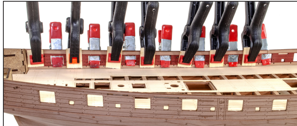
159. Now do the same for part 90R, seen here after gluing and clamping. You may need to trim this slightly at the rear so that it fits flat along the whole length.
