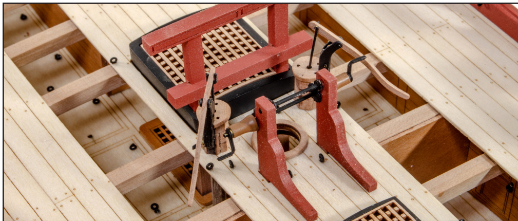
364. Cut two lengths of 3mm dowel 40mm long. Use these to attach the pumps to the deck so that the bottom of the dowel sits into the holes in the lower deck.
