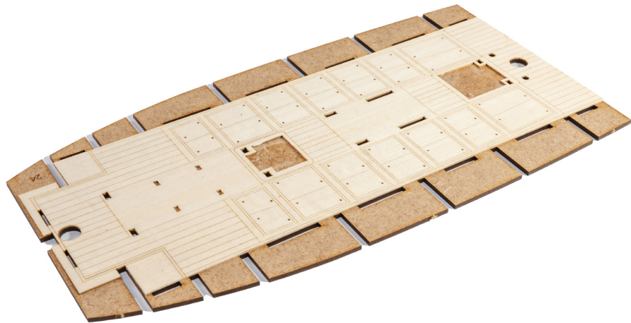
23. The MDF part is engraved with the position on the lime deck, plus you obviously need to line up the various holes. Use wood glue to attach the engraved deck to the MDF and weight the assembly until dry so that the deck won't curl at the edges.
