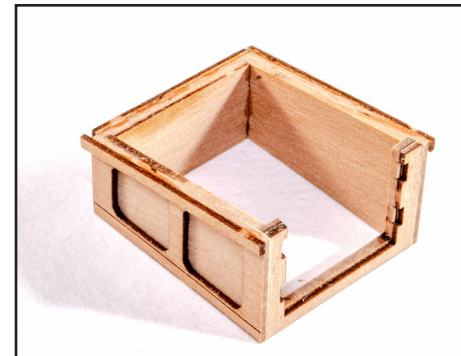
275. Glue part 55 to the top rear of the companionway and when dry, sand the ends flush. Now add parts 54 to the upper sides.
