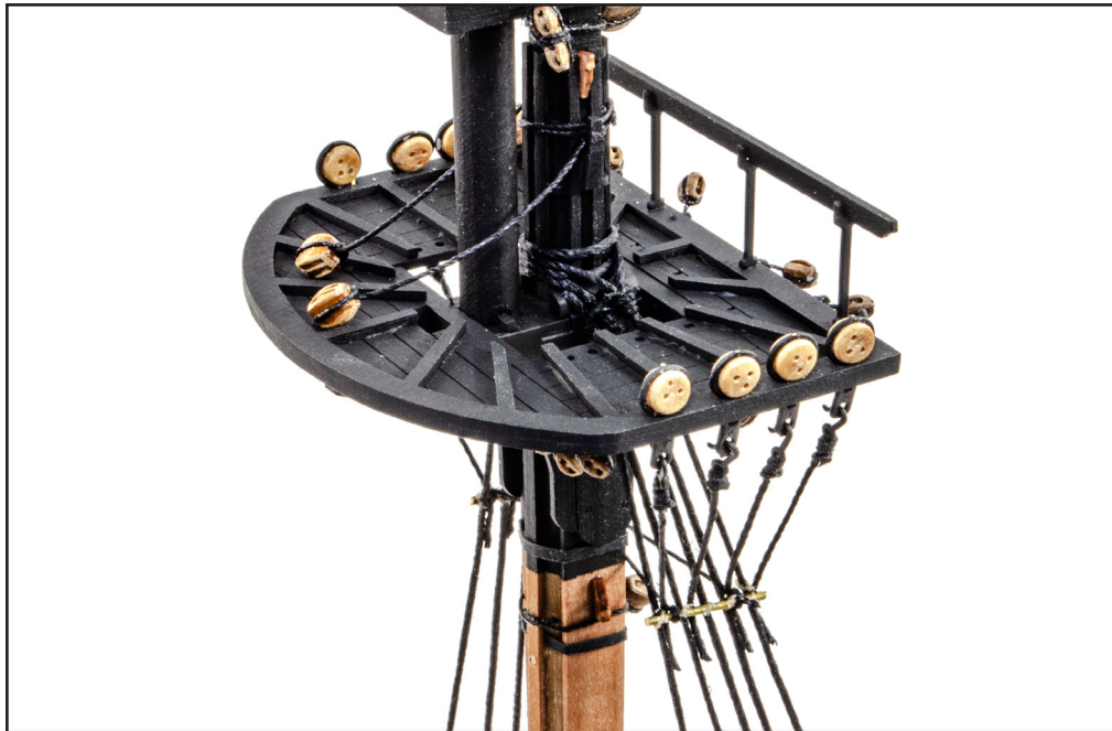
476. Add the 3mm deadeyes to the mast tops and then rig the futtock shrouds into them as shown on the plan.
