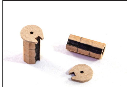
357. To the top of each pump body, glue a part 162, from the 1mm wood sheet. Again, make sure the recess is aligned with those on the pump bodies.
