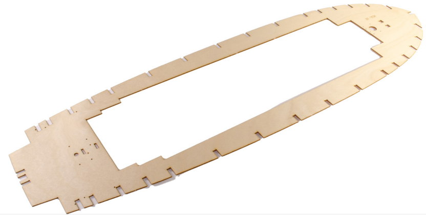
101. With the lower deck complete, we can move upwards. From the 0.8mm ply sheet, remove part 37.
