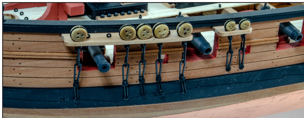
408. These assemblies now need to be slipped into the holes on the channel, noting specifically where the 5mm and 3mm deadeyes need to fit. From the 0.4mm PE sheet, remove all the chainplate parts PE-19, PE-20, PE-21, PE-23, and PE-24, putting them into tubs for each specific part number. Now follow the plan sheet and add these chainplate links to the deadeye assemblies and securing to the hull using brass pins. From the 0.4mm PE sheet, also remove parts PE-14 and glue these eyelets to the channels as seen here and on plans. We find it best to prime and pre-paint these parts before assembly
