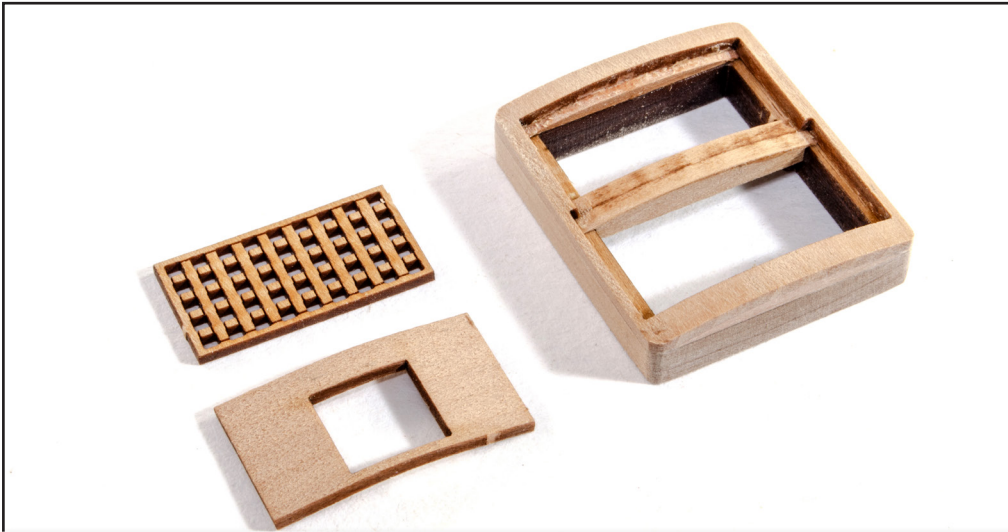
297. The forward hatch assembly also has another curved that needs to be curved and then glued into place, following the same procedure as before. For the forward hatch, this part can be found on the 1mm wood sheet and is part 155. The grates for the assemblies shouldn't need to be soaked to fit easily. For this forward assembly, you will need part 154 on the 1mm wood sheet.
