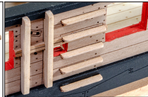
227. Glue the steps into place in the engraved areas as shown. One step will also be fastened to the wale, in the same sequence as the others.
